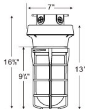
VP102A-C (Ceiling Mount)
