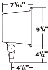
1/2"NPT Swivel
