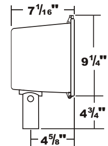
Yoke Mount
